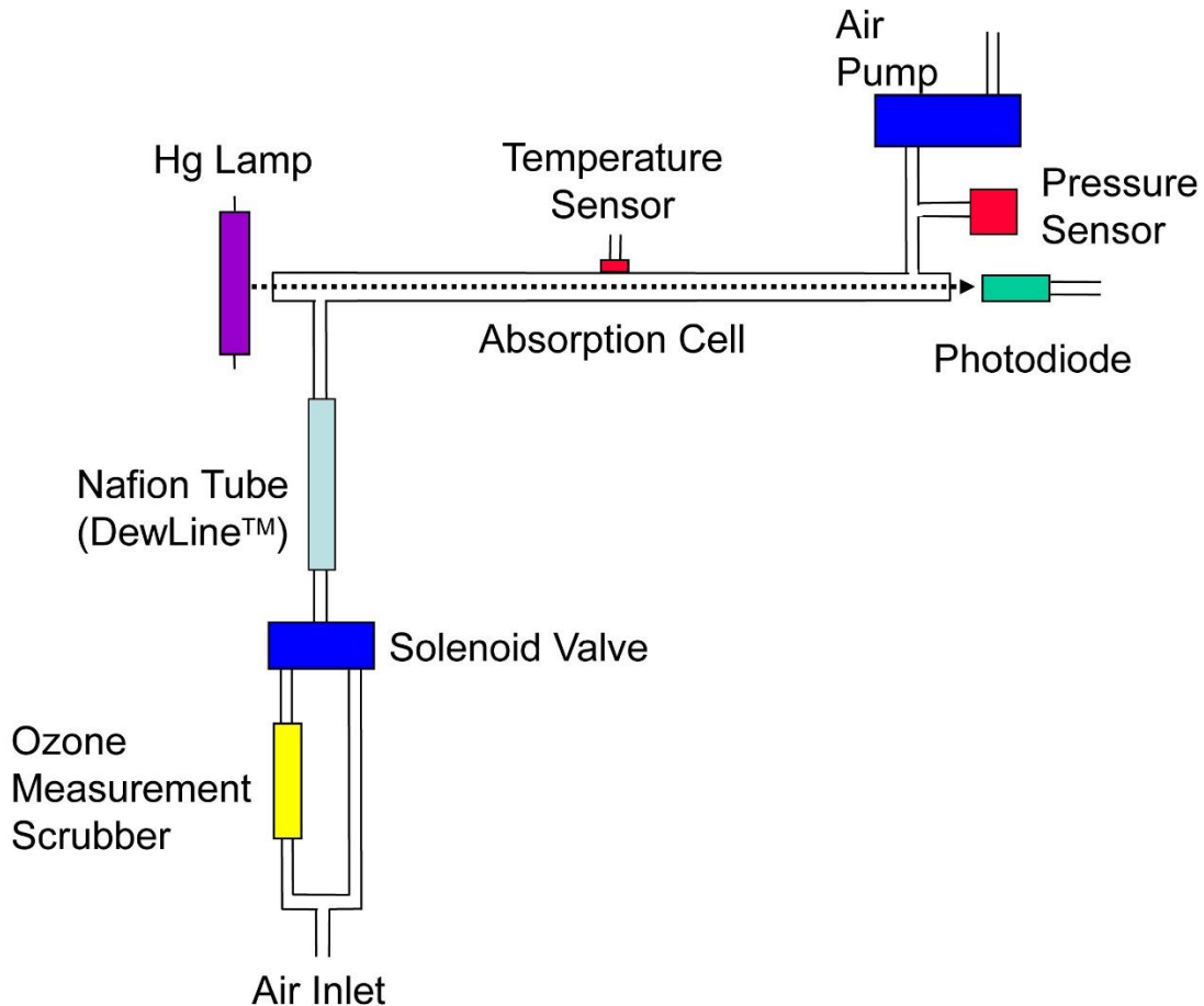
Figure 1.1. Schematic Diagram of the Ozone Monitor.
