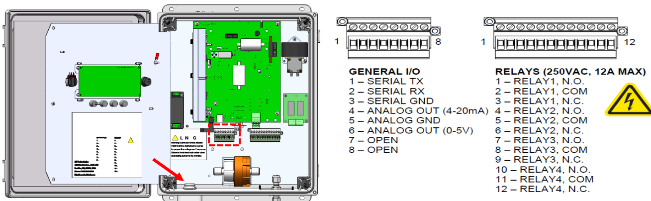
Figure D-5. Serial connections and analog connections (red dashed box) and relay connections (red solid box) to the Multi-Channel 106. Route connecting wires through the power/serial/relays port (red arrow).
