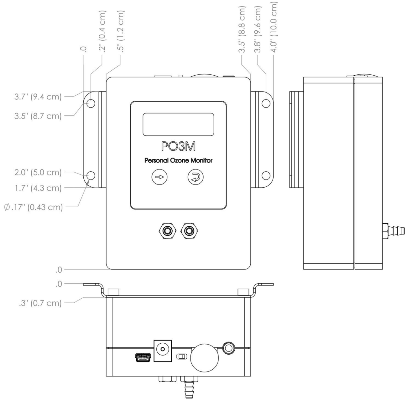
Figure 3. Dimensions of the POM with wall mounting bracket.
