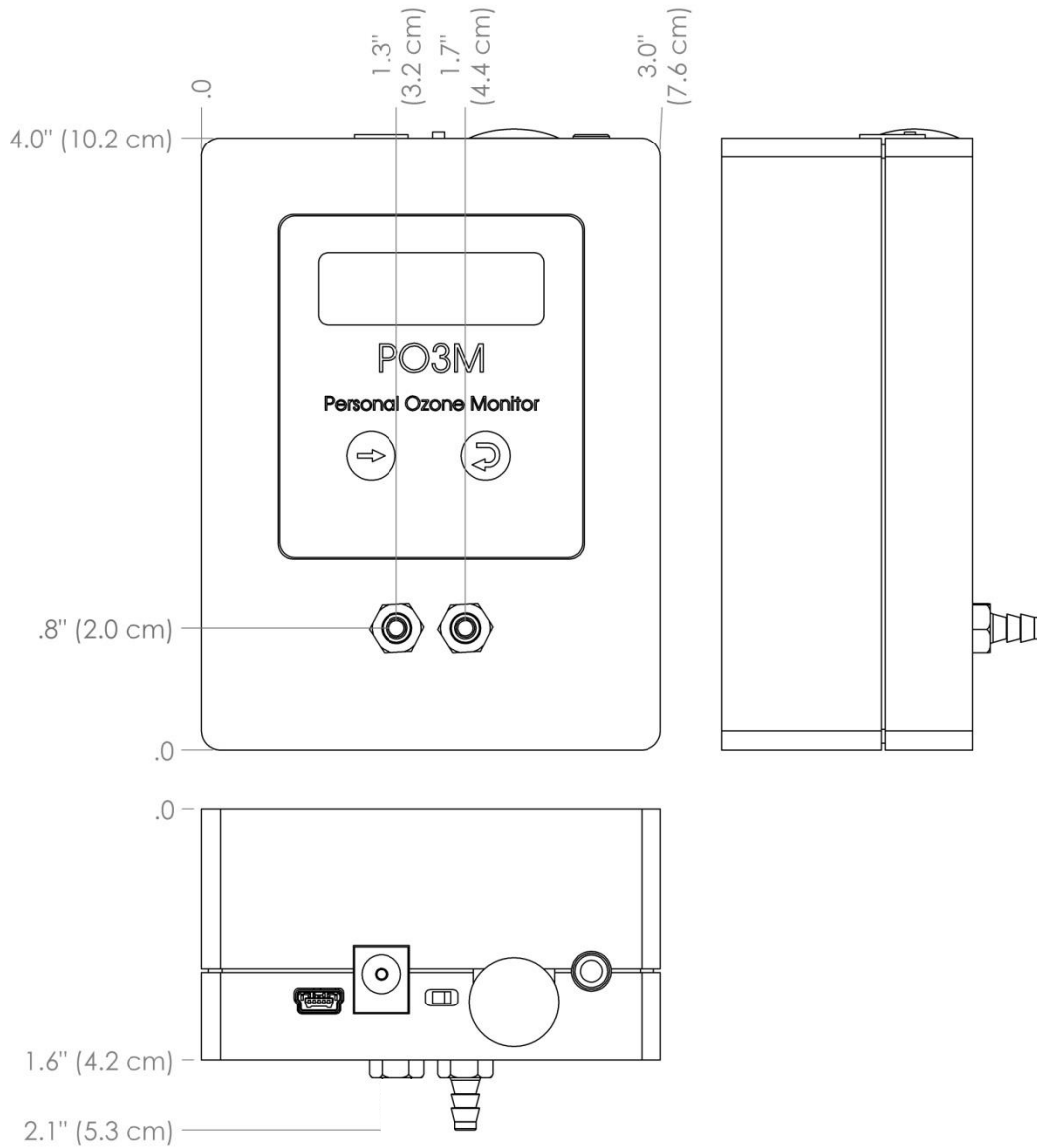
Figure 1. Dimensions of the POM.
