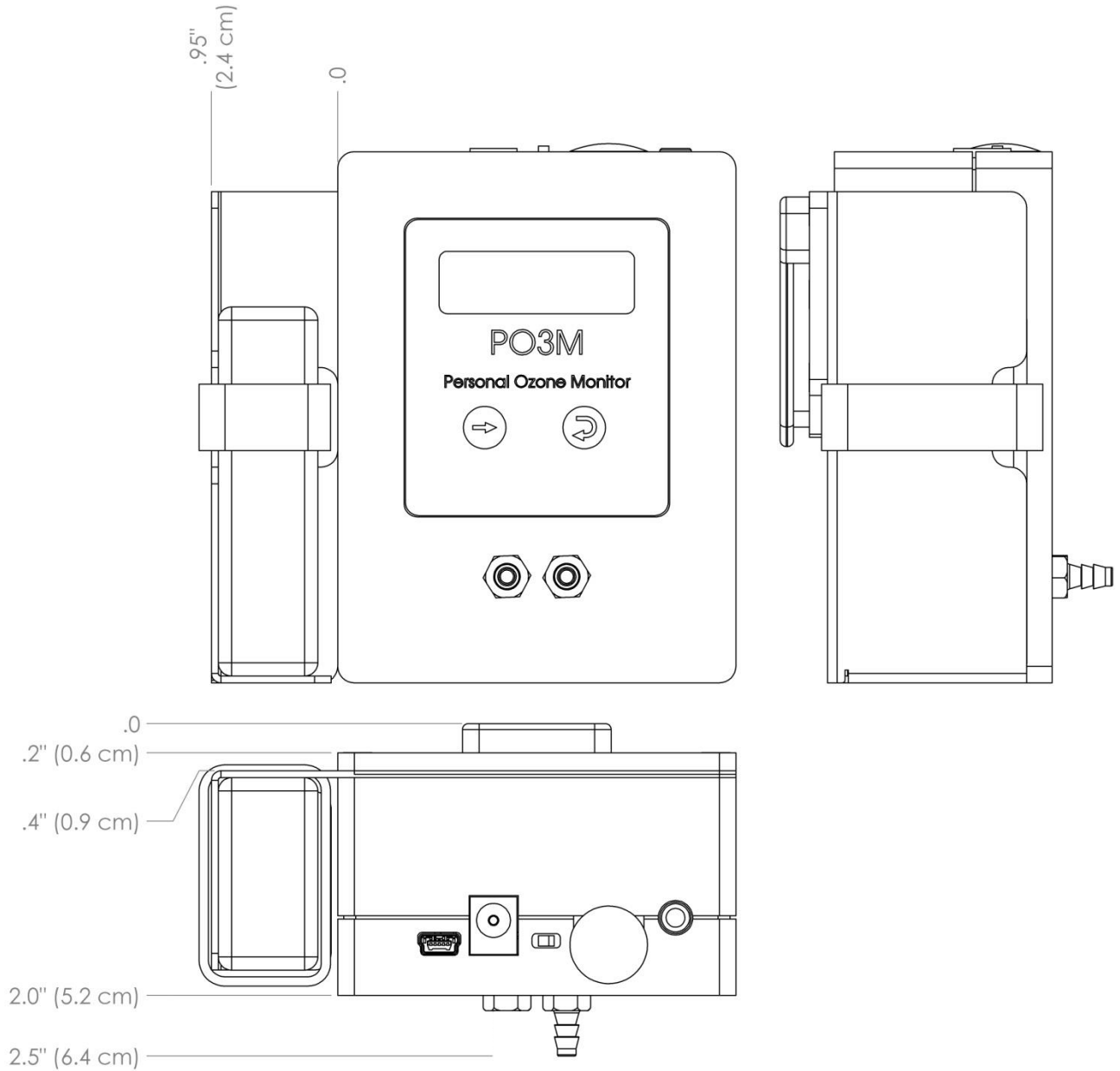
Figure 2. Dimensions of the POM with battery bracket and battery.
