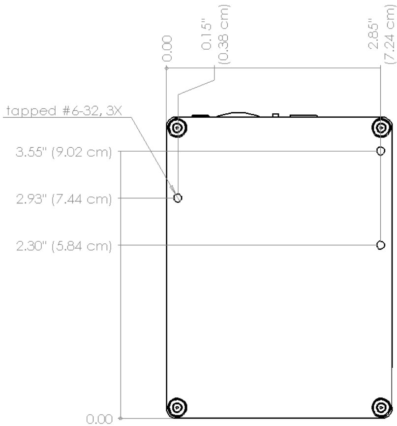
Figure 4. Mounting holes on the back of the POM.
